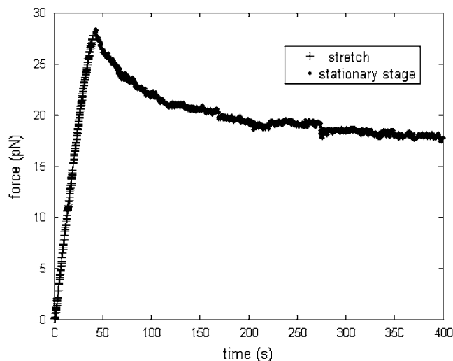
FIGURE 4 Within the first 40 \text{ seconds} , a tether is extracted from the rough strain S2188 to a distance of 4 \mu\text{m} with a velocity of 0.1 \mu\text{m/s} . At this extreme position the stage is stopped and the figure shows how the force in the tether relaxes as a function of time.
